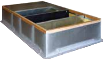
Roof-top unit replacements from popular manufacturers using adapter curbs
